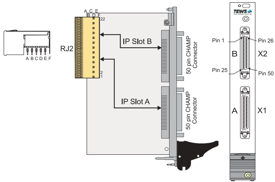
Figure 6-1 : Pin Assignment
