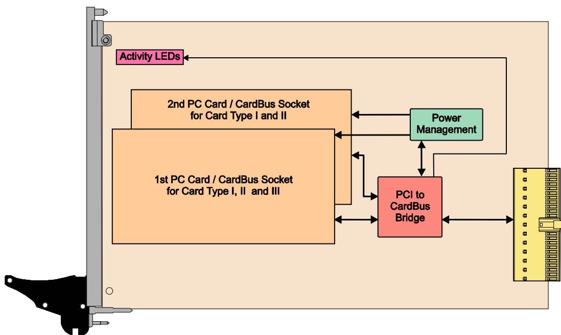
Figure 1-1 : Block Diagram
