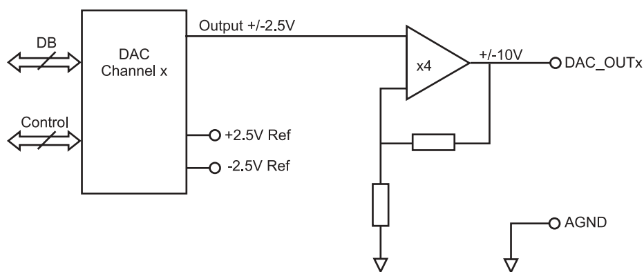
Figure 5-4 : Output Wiring
