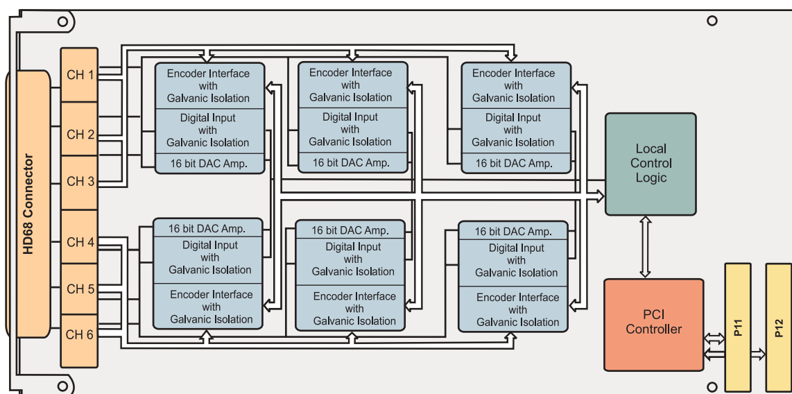
Figure 1-1 : Block Diagram
