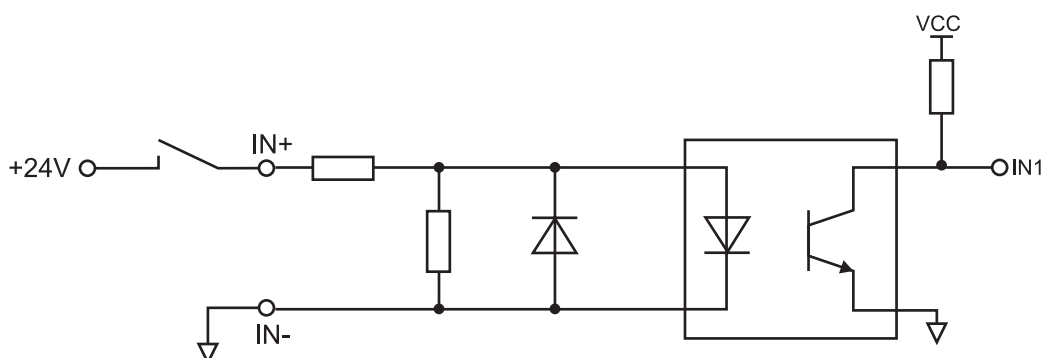
Figure 5-3 : Input Wiring
