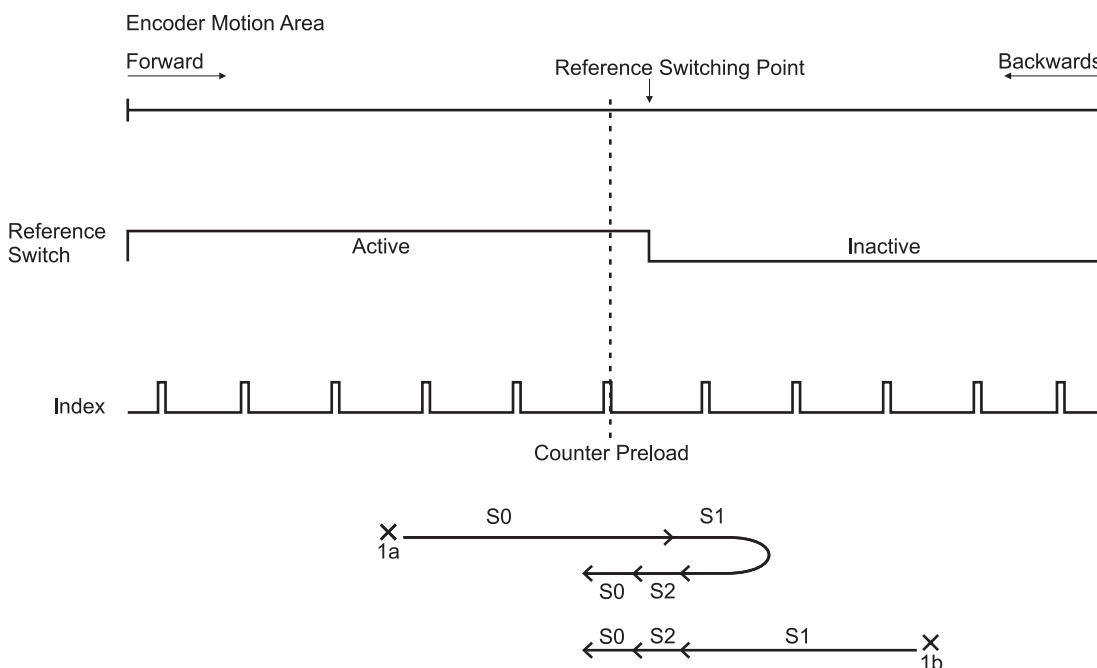
Figure 3-6 : Encoder preload example
