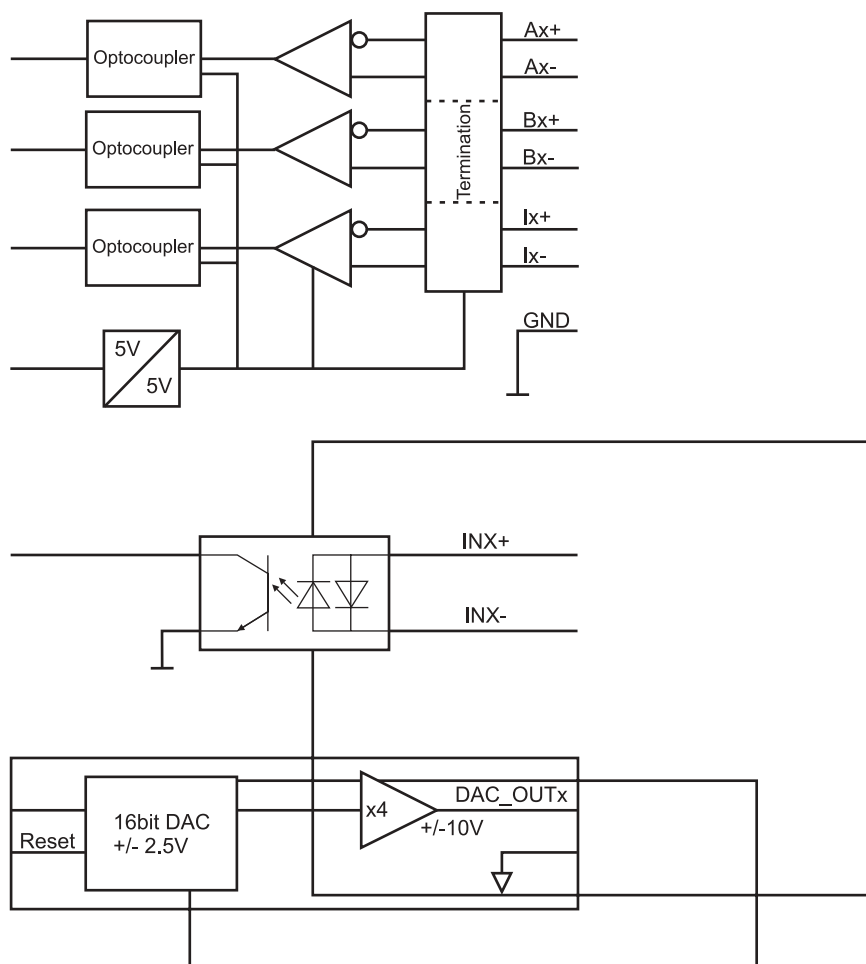
Figure 5-1 : Detailed Motion Control Channel
