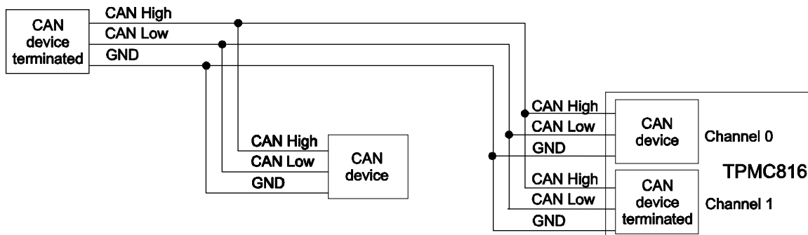
Figure 6-3 : Typical operating circuit
