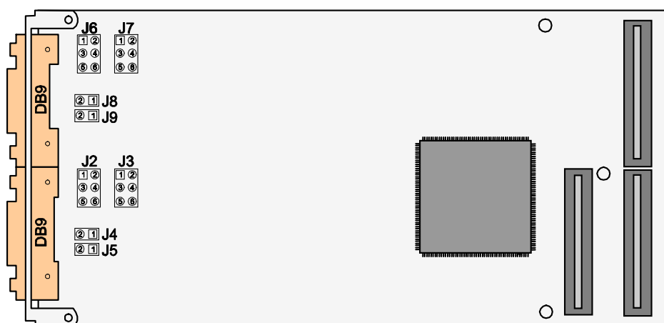
Figure 6-2 : Jumper Location TPMC816
