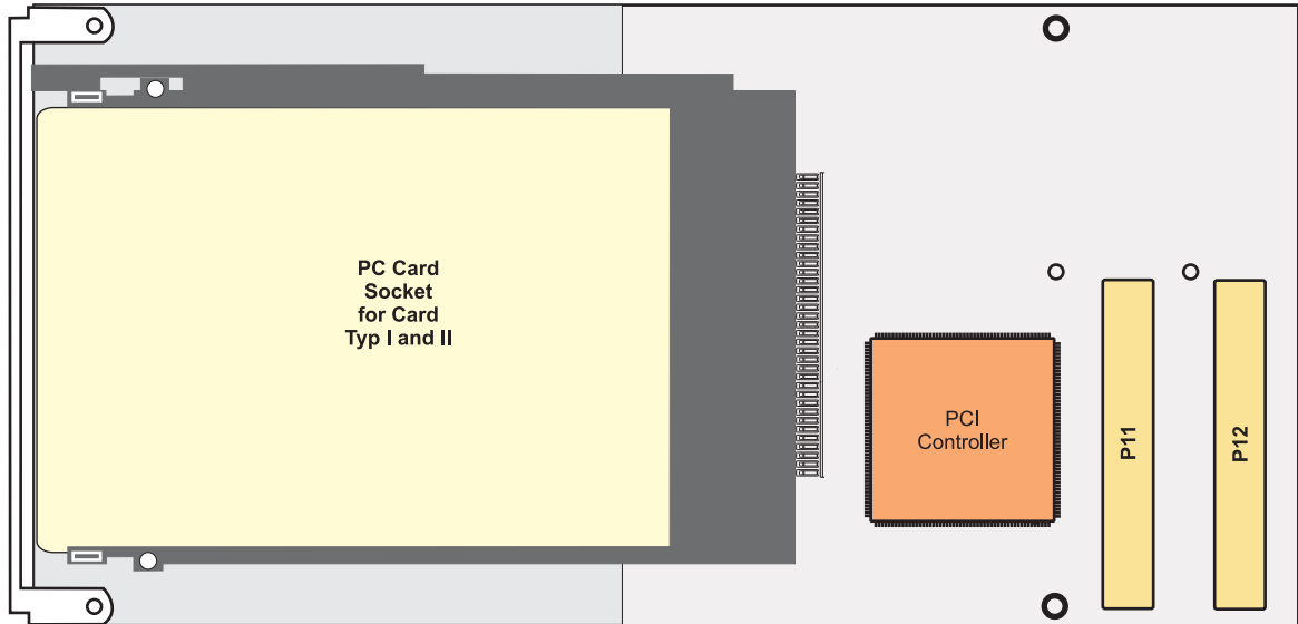
Figure 1-4 : Module TPMC871-50
