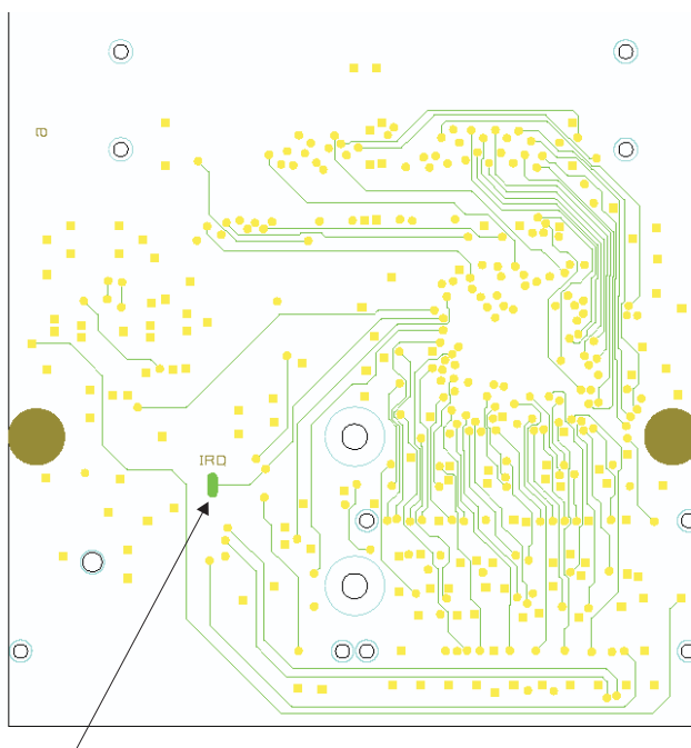
MFUNC3 ISA IRQ signal can be accessed here
