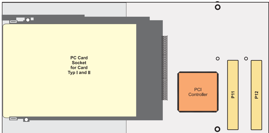
Figure 1-3 : Module TPMC871-11
