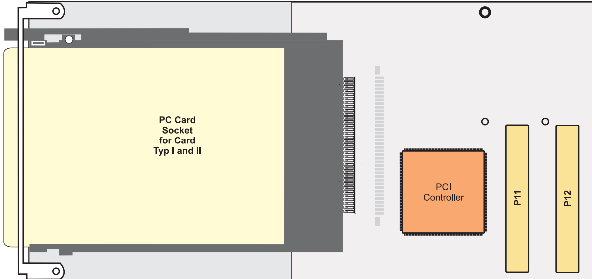
Figure 1-2 : Module TPMC871-10
