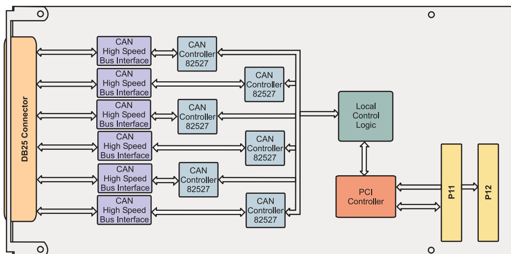
Figure 1-1 : Block Diagram
