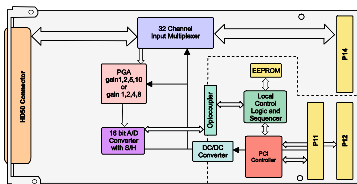
Figure 1-1 : Block Diagram
