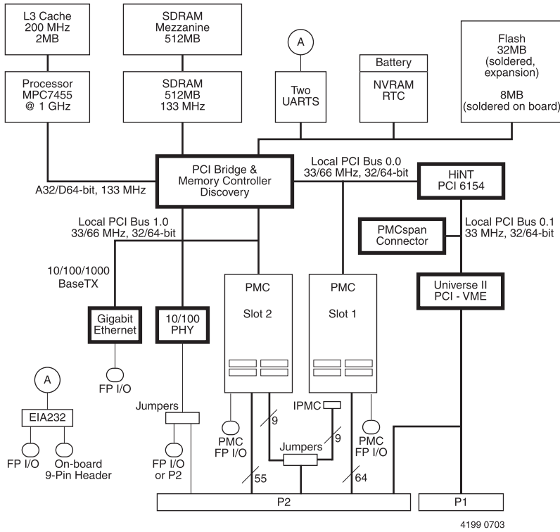
Figure 1-1. MVME5500 Block Diagram
