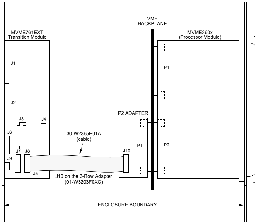
Figure 2-5. MVME761EXT 10Mbps Ethernet Connection
