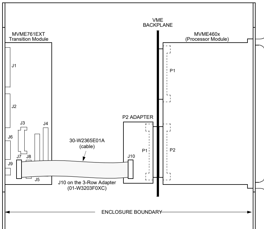
Figure 2-6. MVME761EXT 10/100 BaseT Connection
