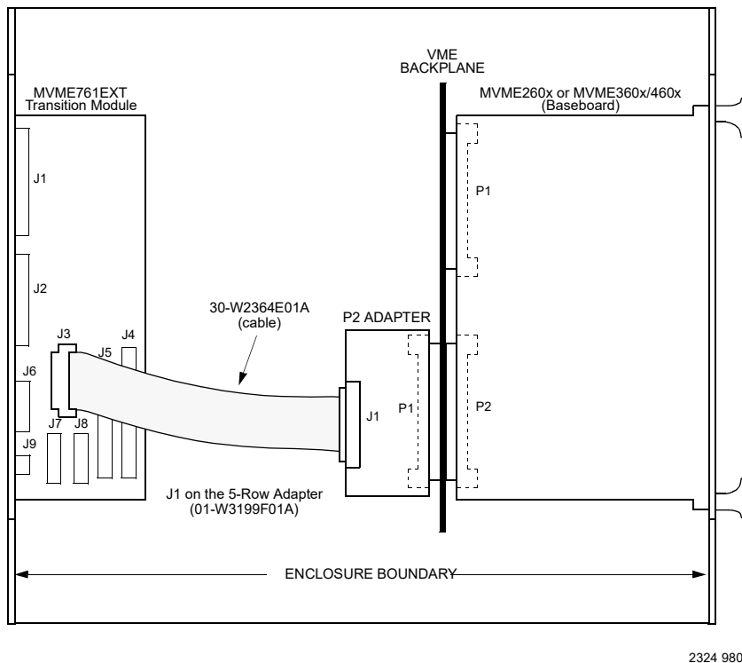
Figure 2-2. MVME761EXT 8/16 bit Single Ended SCSI Connection
