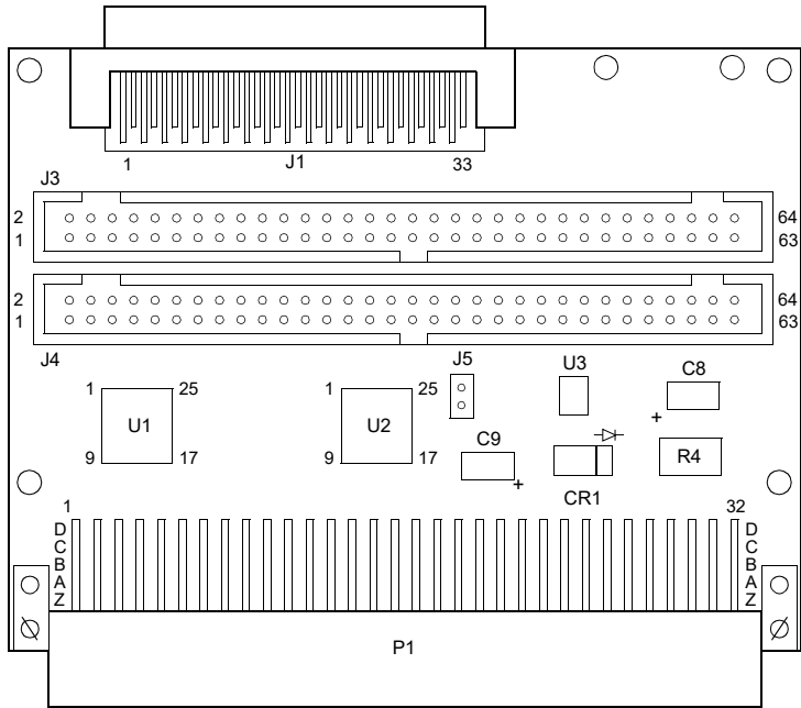
Figure 1-4. 5-row DIN Backplane P2 Adapter (MVME761EXT)
