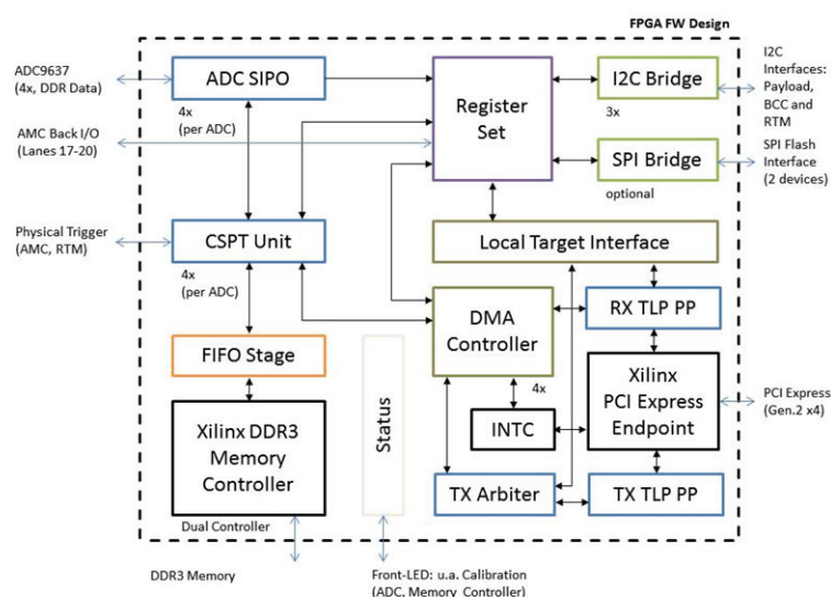
Figure 6-1 : TAMC532 Firmware SOC Structure
