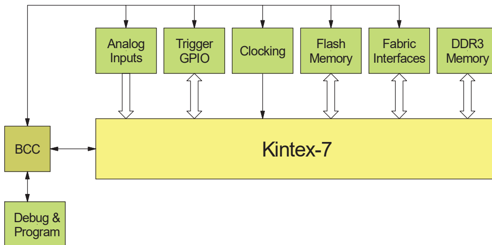
Figure 5-1 : Functional Block Diagram
