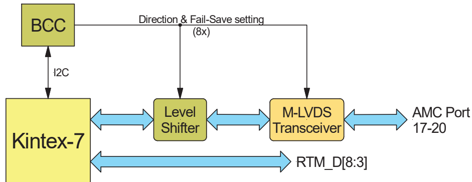
Figure 5-6 : M-LVDS I/O
