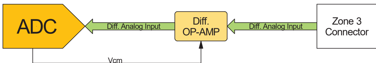
Figure 5-7 : Single Analog Input
