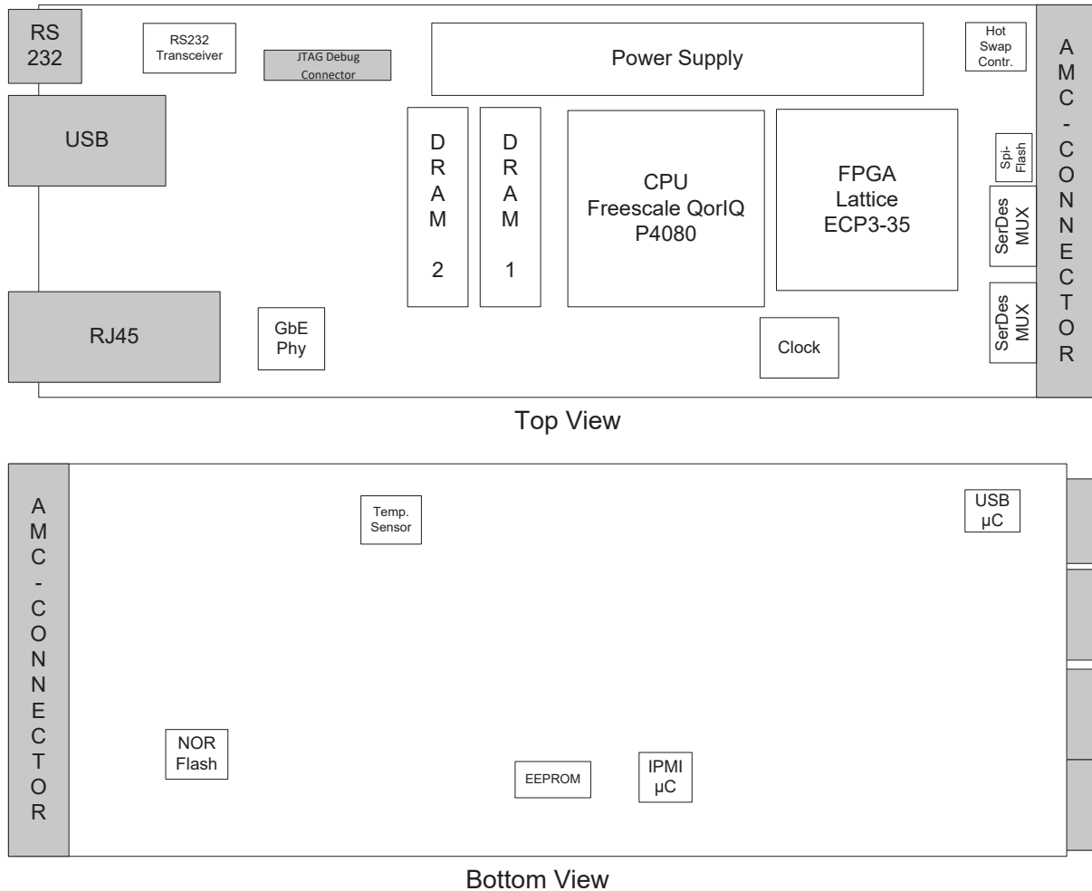
Figure 7: NAMC-QorIQ-P4080-ECO – Location Diagram – Overview
