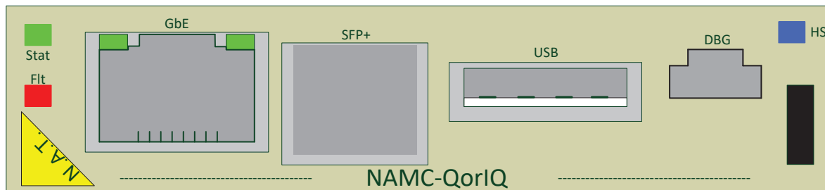
Figure 10: NAMC-QorIQ-P4080 – Front Panel View
