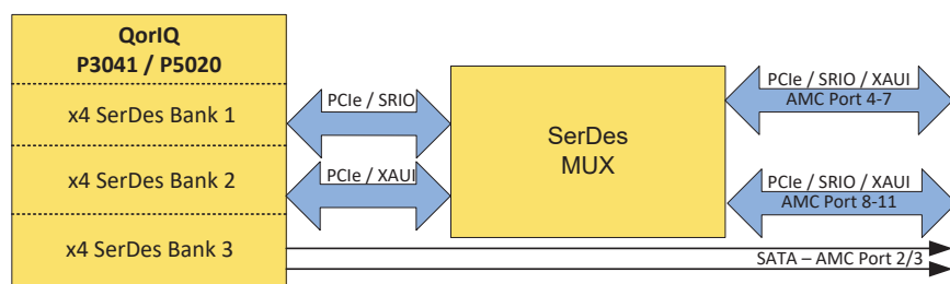
Figure 9: NAMC-QorIQ-P3041/P5020 – SerDes Connectivity - Overview
