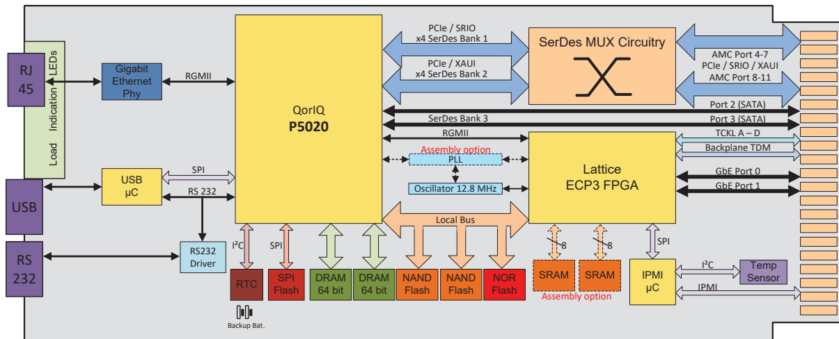
Figure 5: NAMC-QorIQ-P5020 – Block Diagram – Overview
