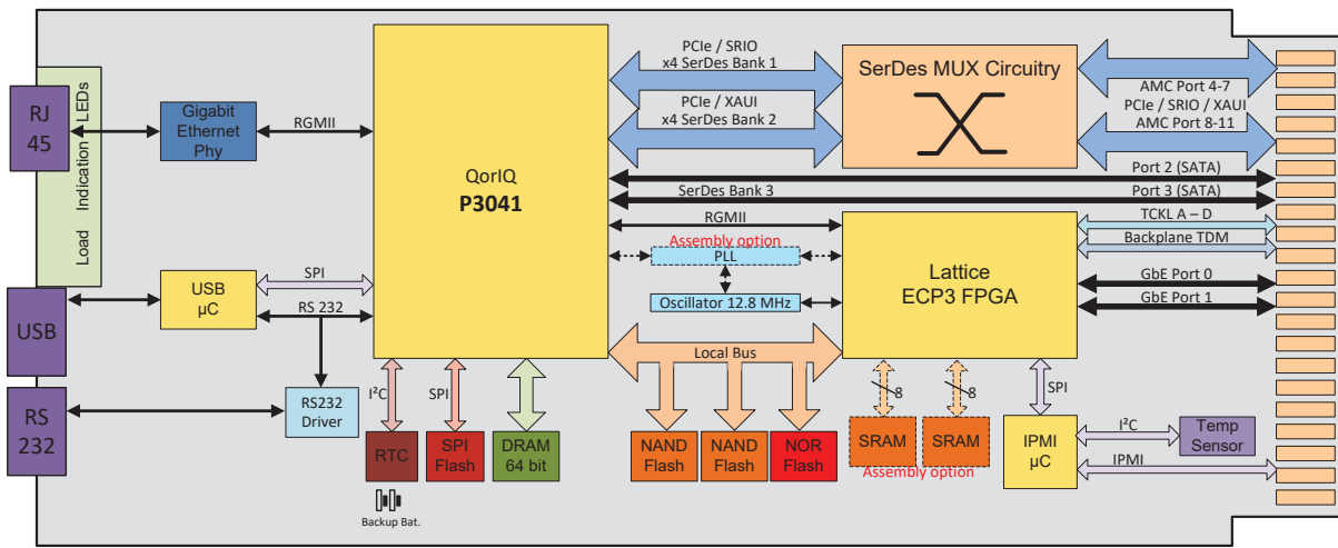
Figure 2: NAMC-QorIQ-P3041 – Block Diagram – Overview
