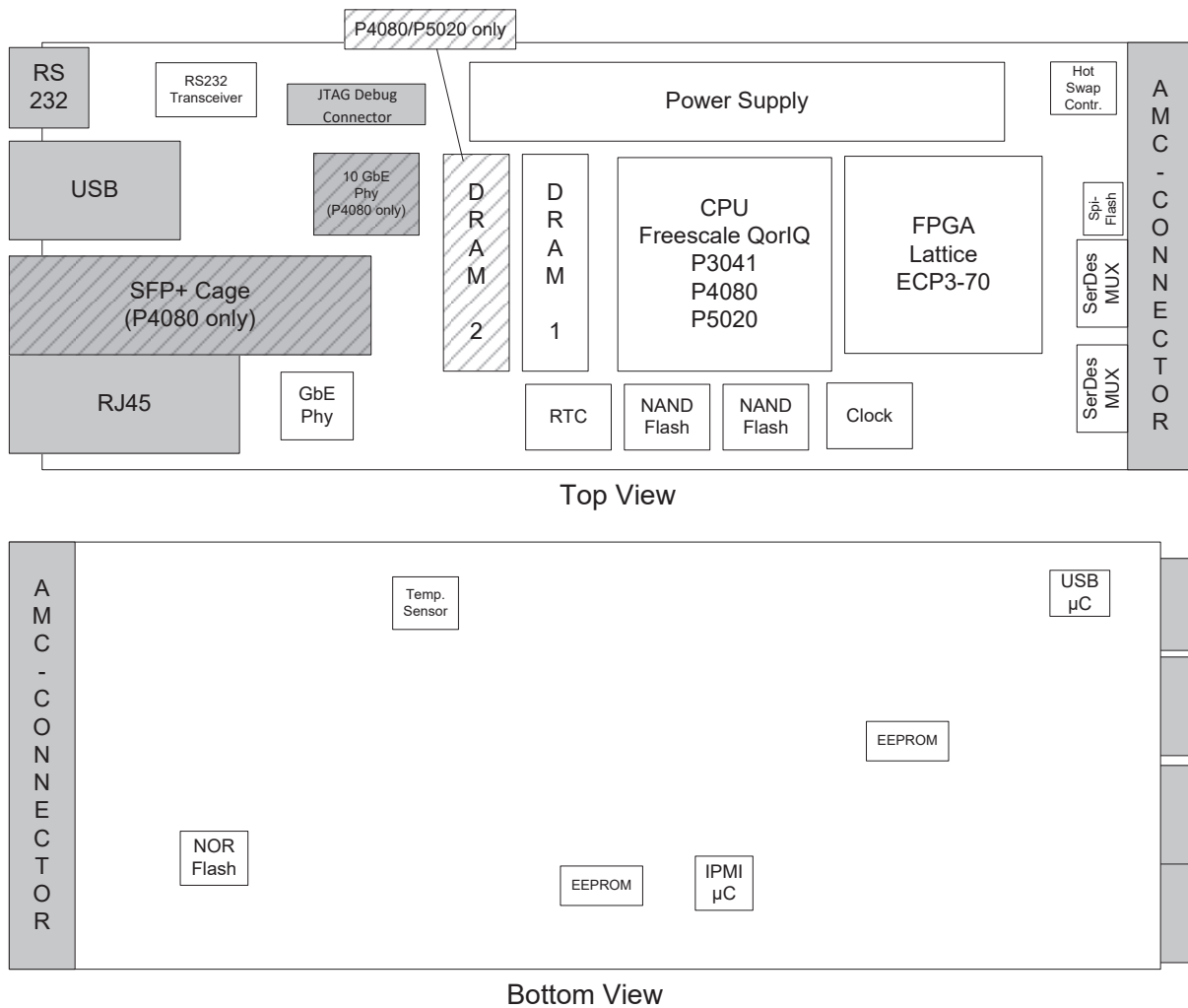
Figure 6: NAMC-QorIQ-Pxxx – Location Diagram – Overview
