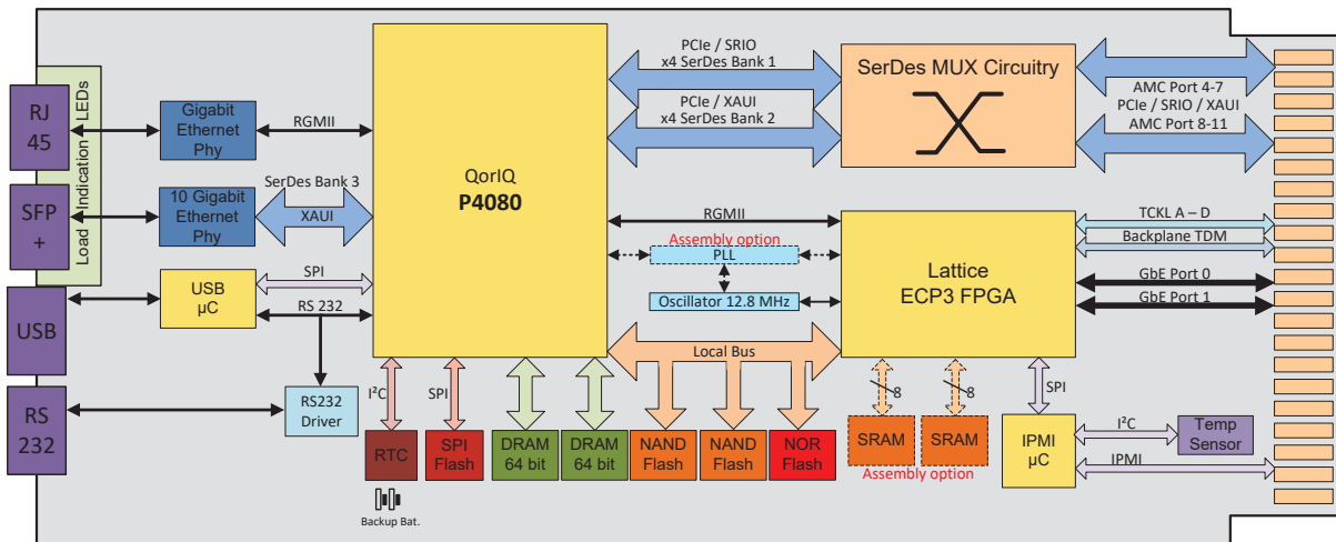
Figure 3: NAMC-QorIQ-P4080 – Block Diagram – Overview
