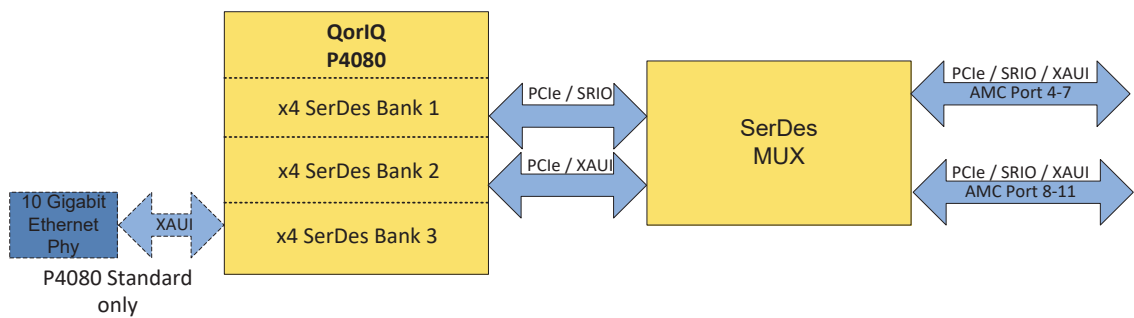
Figure 8: NAMC-QorIQ-P4080 – SerDes Connectivity – Overview
