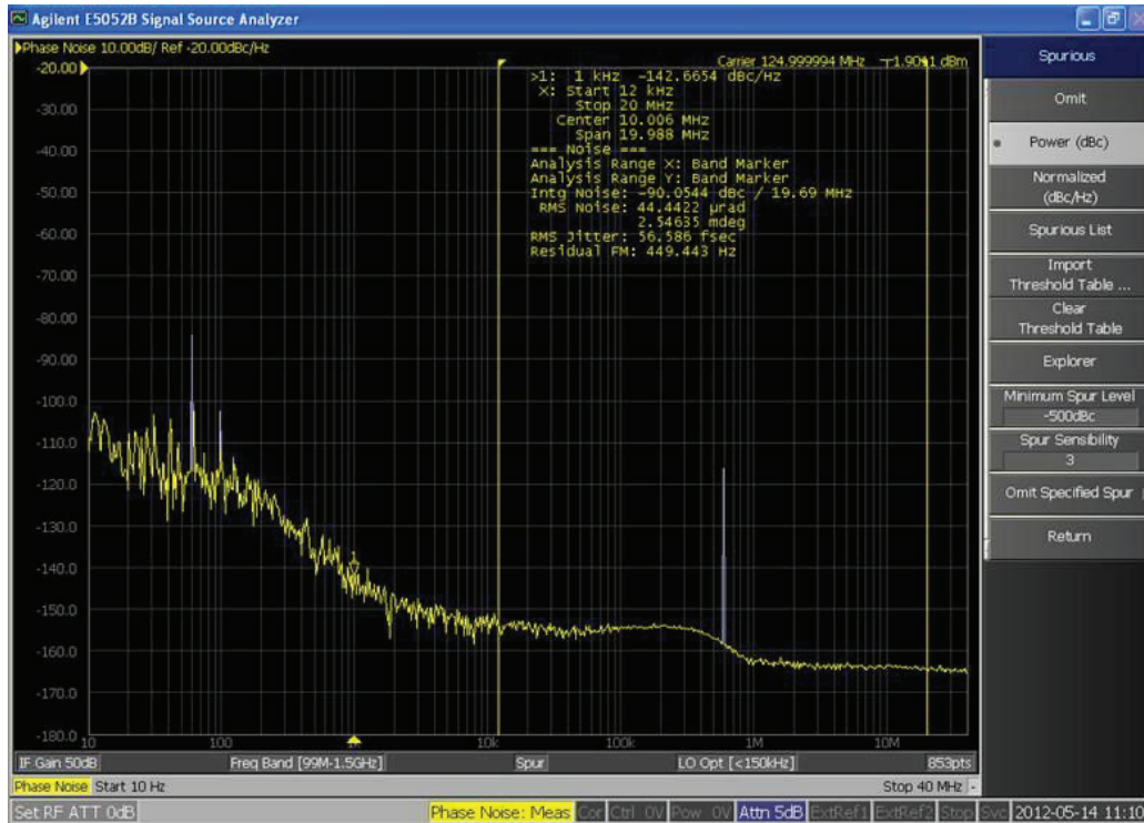
Figure 9: Phase Noise Plot of Input Signal
