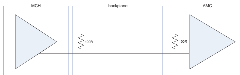
Figure 5: M-LVDS-Termination
