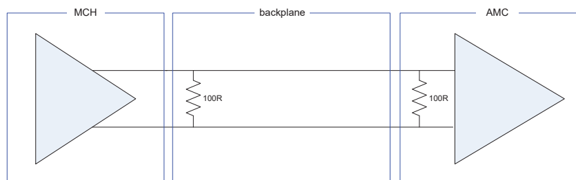
Figure 4: M-LVDS Termination
