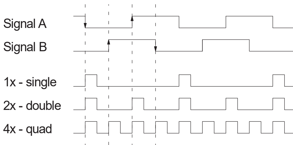
Figure 5-4: Quadrature Signals
