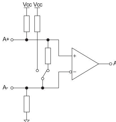
Figure 6-1: Input Wiring
