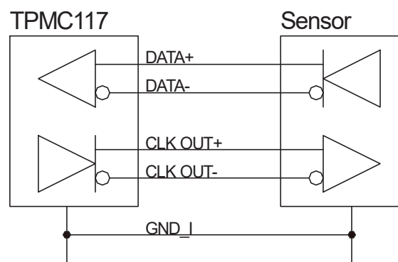
Figure 6-5: TPMC117 Clock Output Wiring
