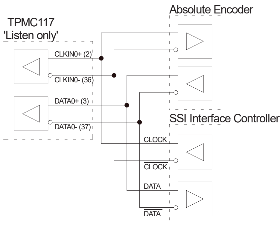
Figure 5-3: Wiring Example: Channel 0, 'Listen only' Mode
