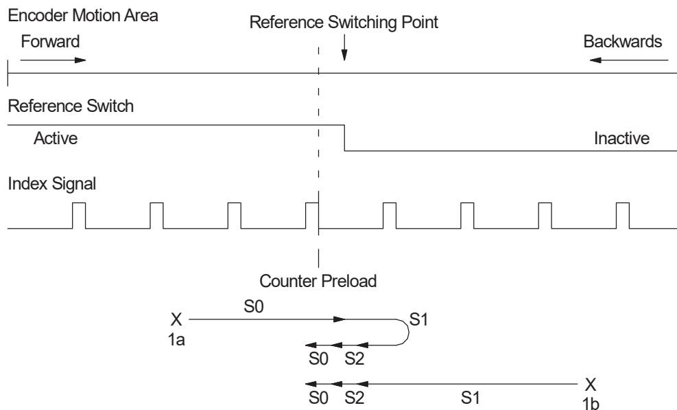
Figure 5-5: Reference mode preload example
