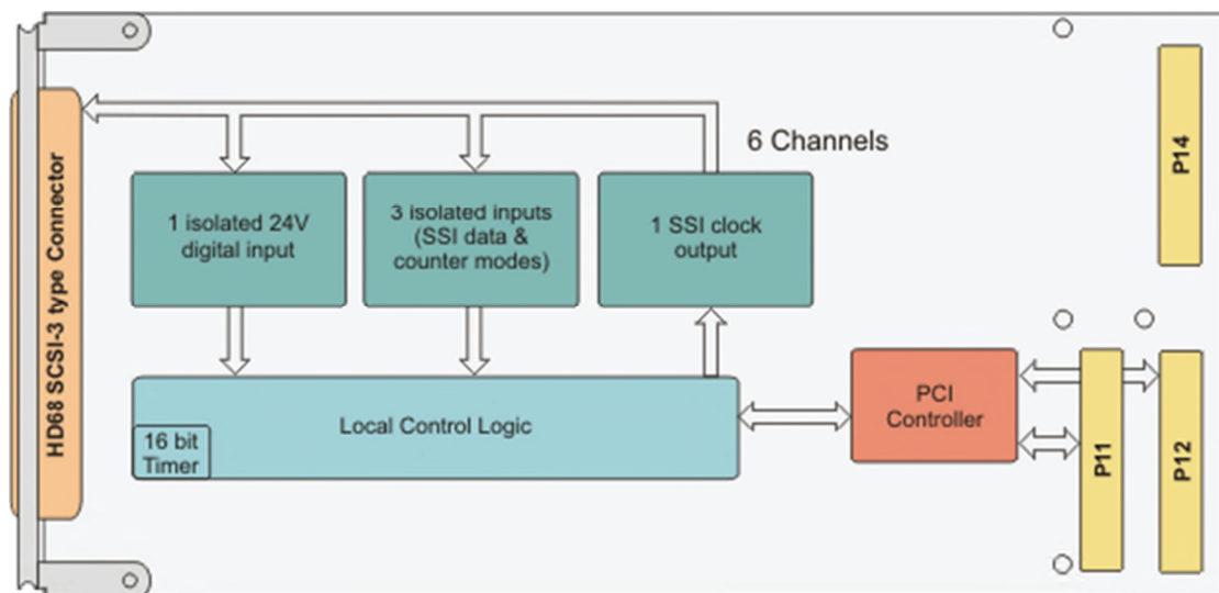
Figure 1-1: Block Diagram
