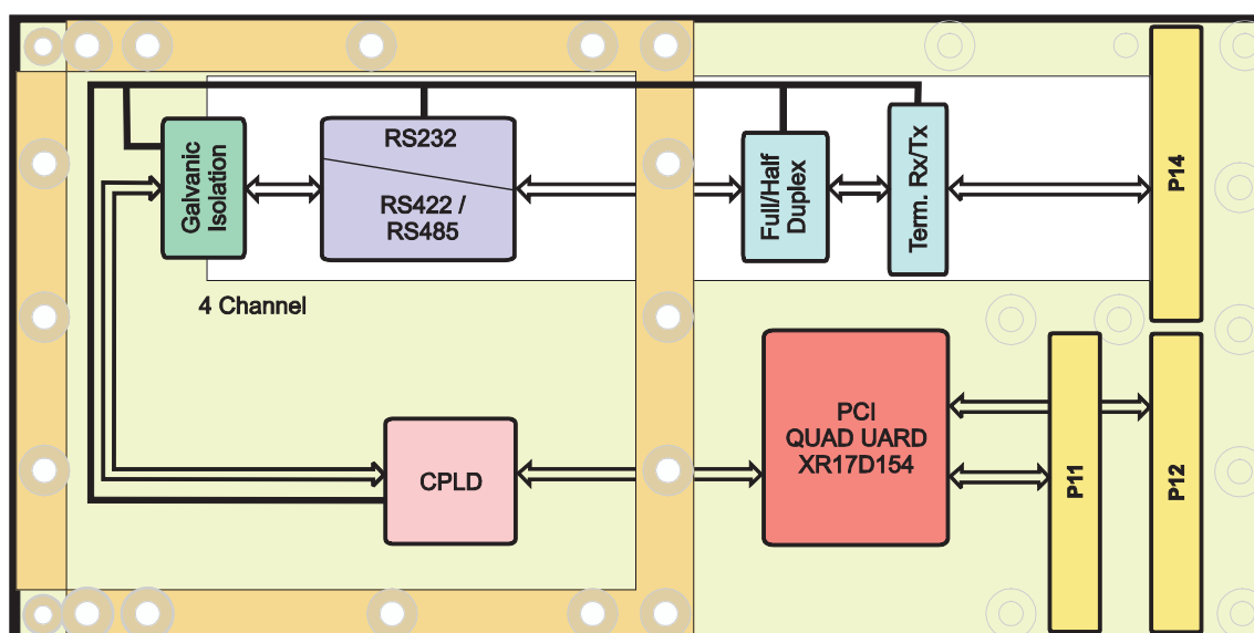
Figure 1-1 : Block Diagram
