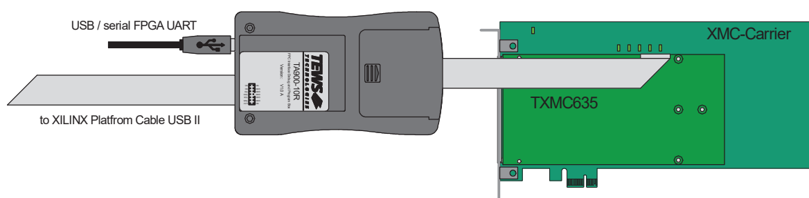
Figure 9-4 : 9.2.1 Connecting TA900 to TXMC635 Debug Connector
