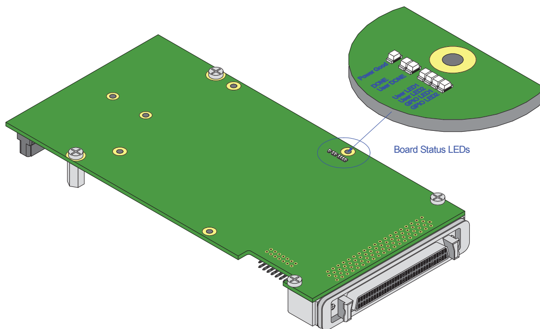
Figure 7-12 : On Board Indicators
