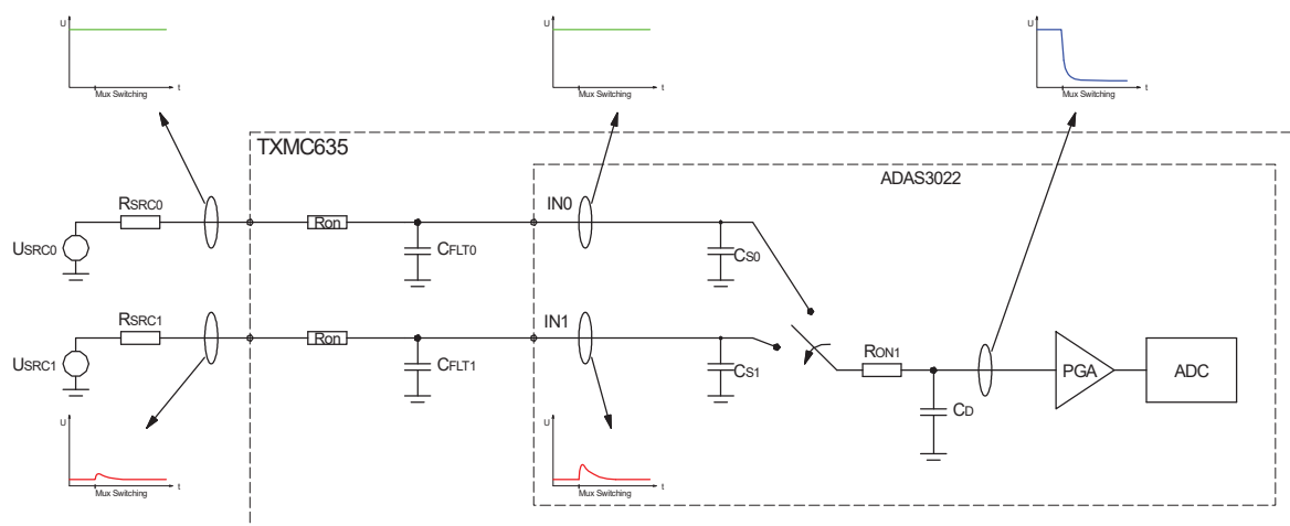
Figure 8-3 : ADAS3022 Mux Switching
