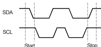
Figure 7-9 : Configuration FPGA Start and Stop condition
