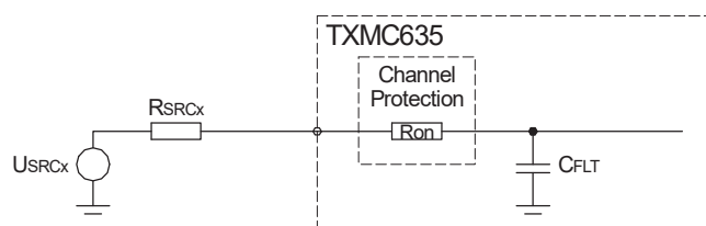
Figure 8-2 : Analog Input filter
