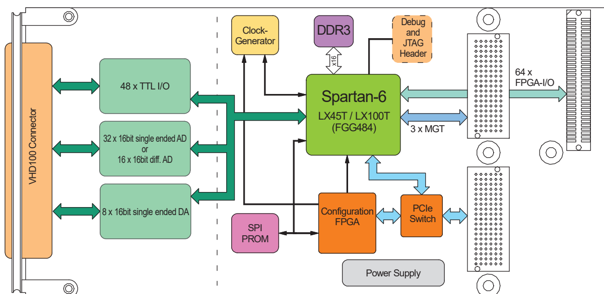
Figure 1-1 : Block Diagram
