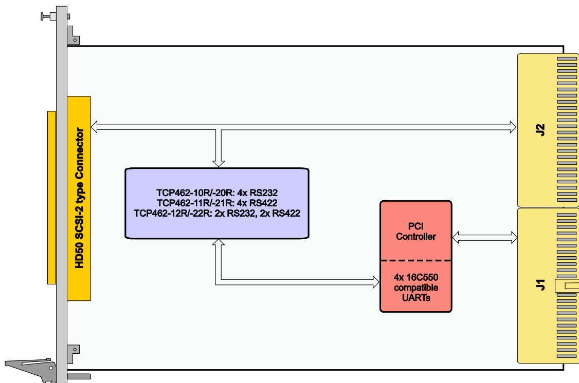
Figure 1-1 : Block Diagram
