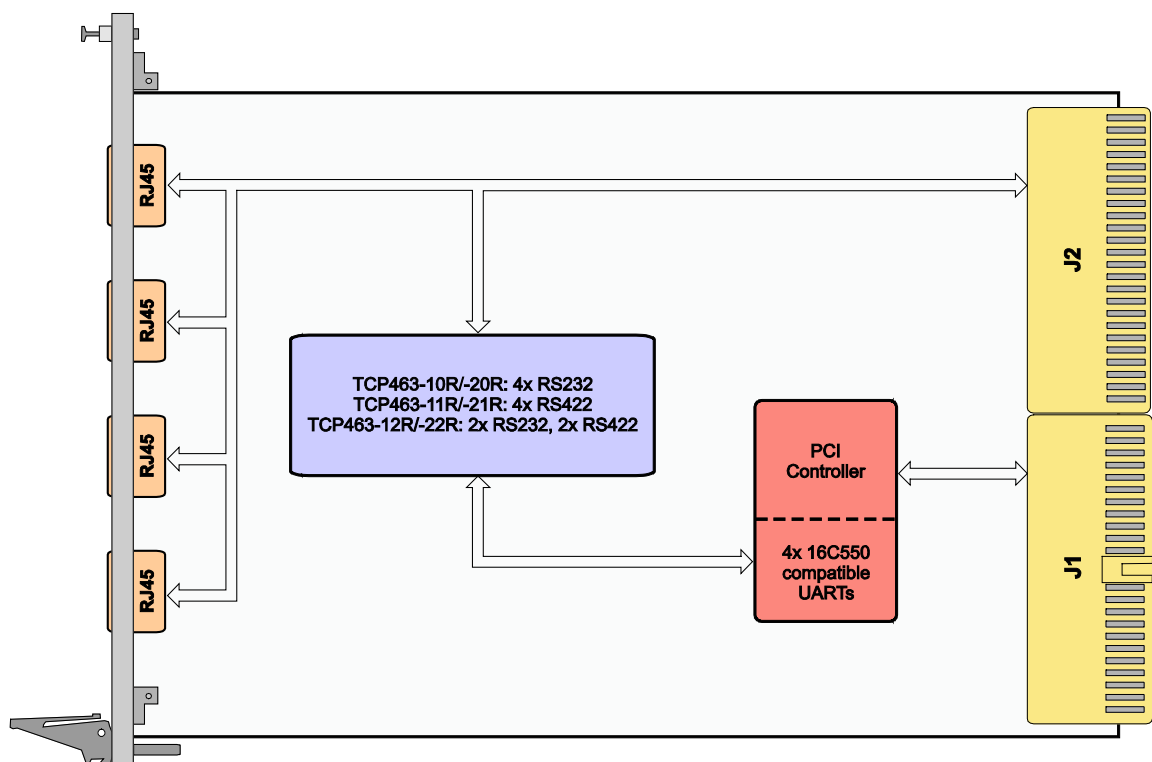
Figure 1-1 : Block Diagram
