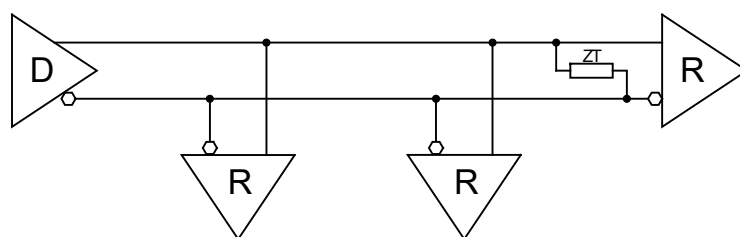
Figure 5-4 : RS422 Multidrop Configuration
