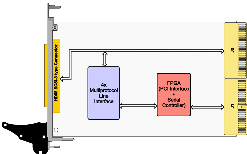
Figure 1-1 : Block Diagram
