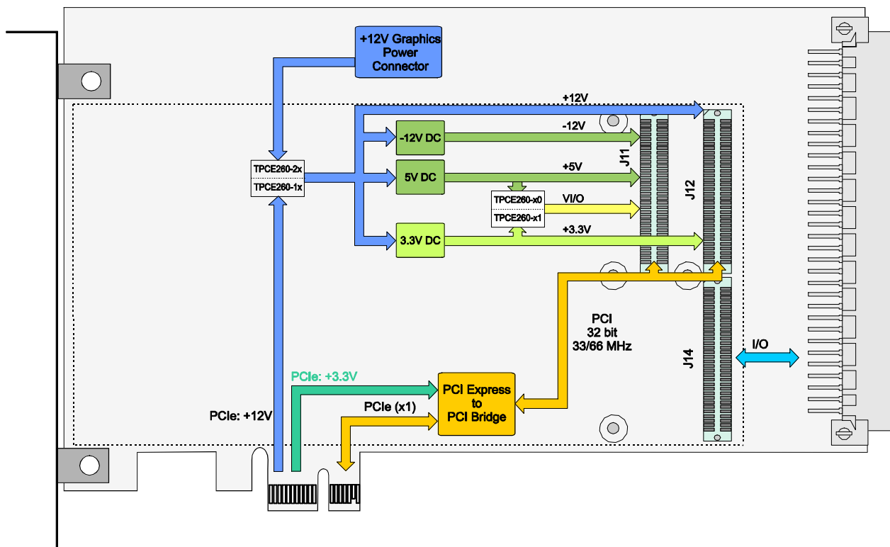
Figure 1-1 : Block Diagram
