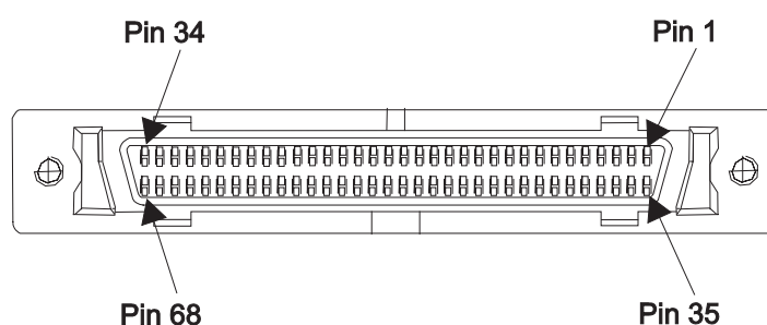
Figure 14-3: Front Panel I/O Connector Numbering
