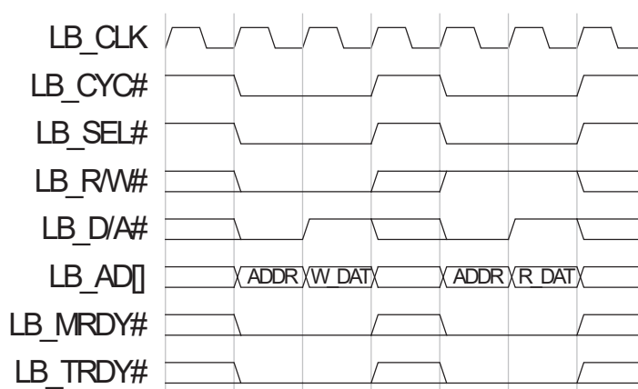
Fast Master Fast Target Local Bus Example
