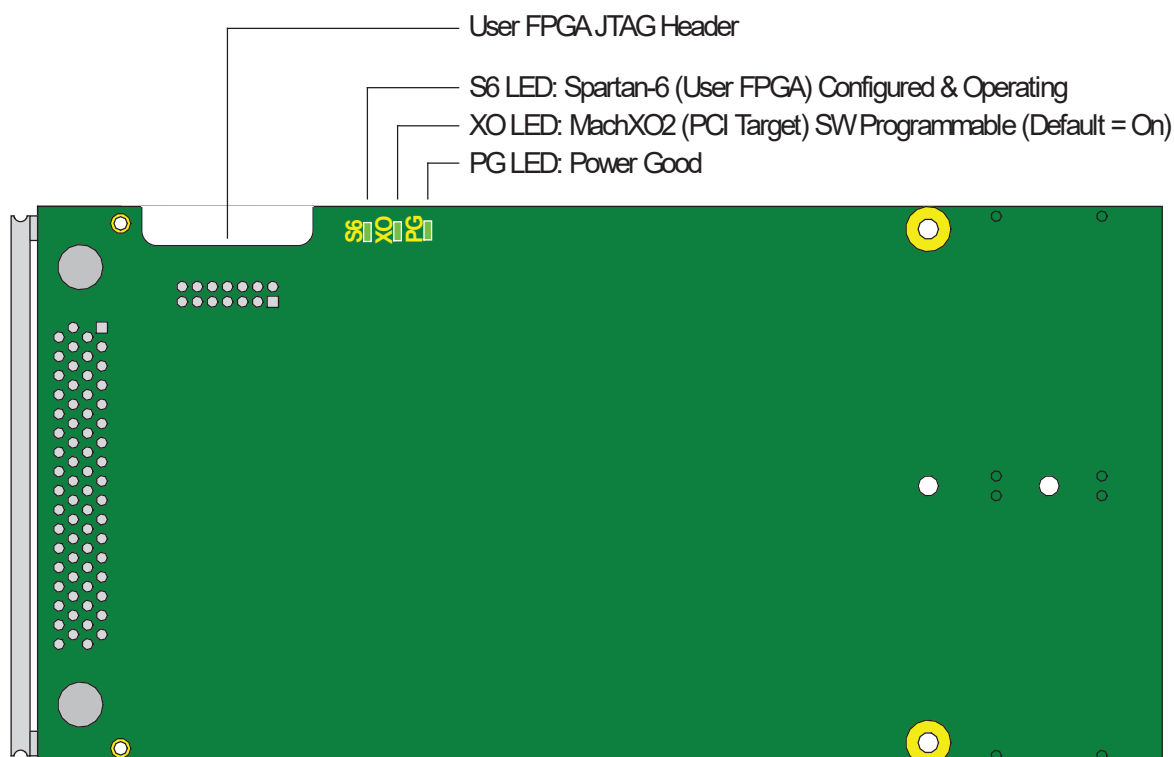
Figure 11-1: LED Location
