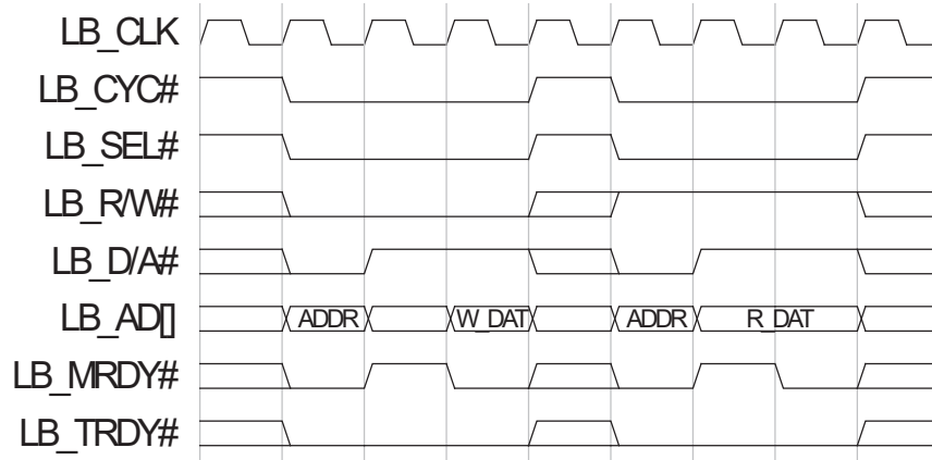
Slow Master Fast Target Local Bus Example
