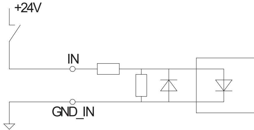
Figure 7-1 : Input Wiring
