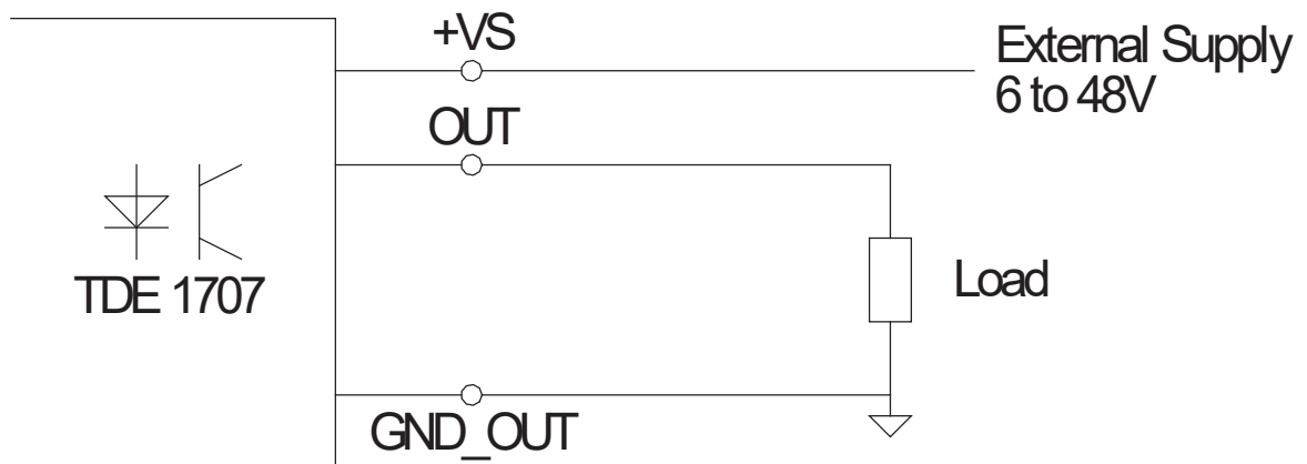
Figure 7-2 : Output Wiring High Side Switch
