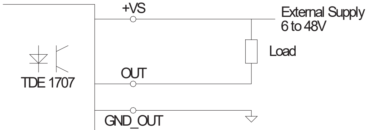
Figure 7-3 : Output Wiring Low Side Switch
