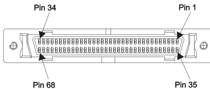
Figure 7-1 : Front Panel I/O Connector Numbering
