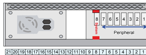
cPCIS-2630R/cPCIS-2830R Inside Rear View
