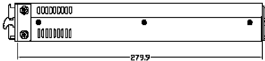
Figure 1-4: cPCIS-6130R Right View
