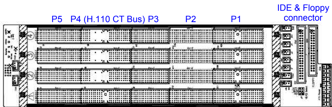
System Slot cBP-6104R Front View
