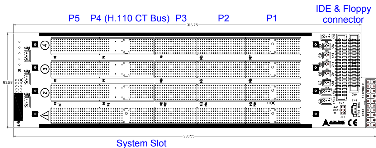
cBP-6404R Front View
