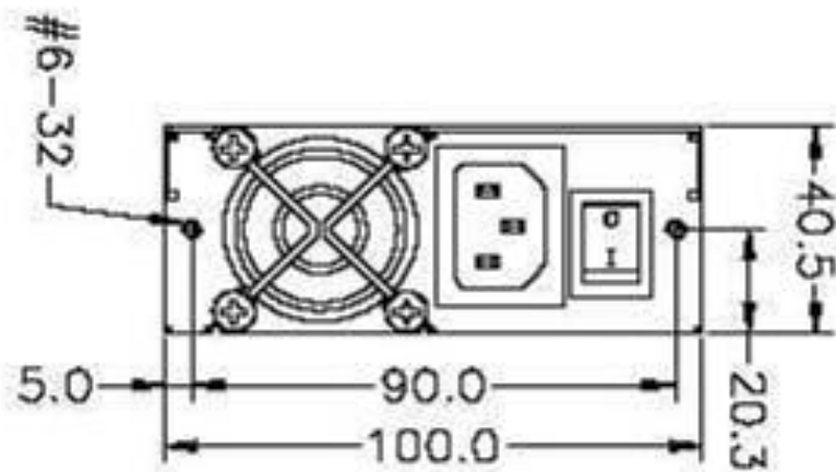
Power Supply Side View
