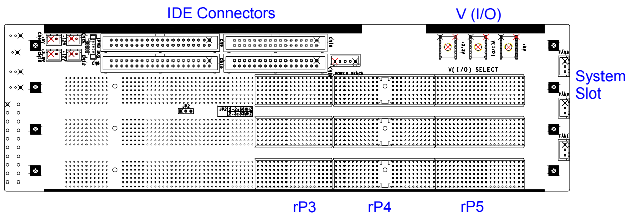
cBP-6403R/N110 Rear View
