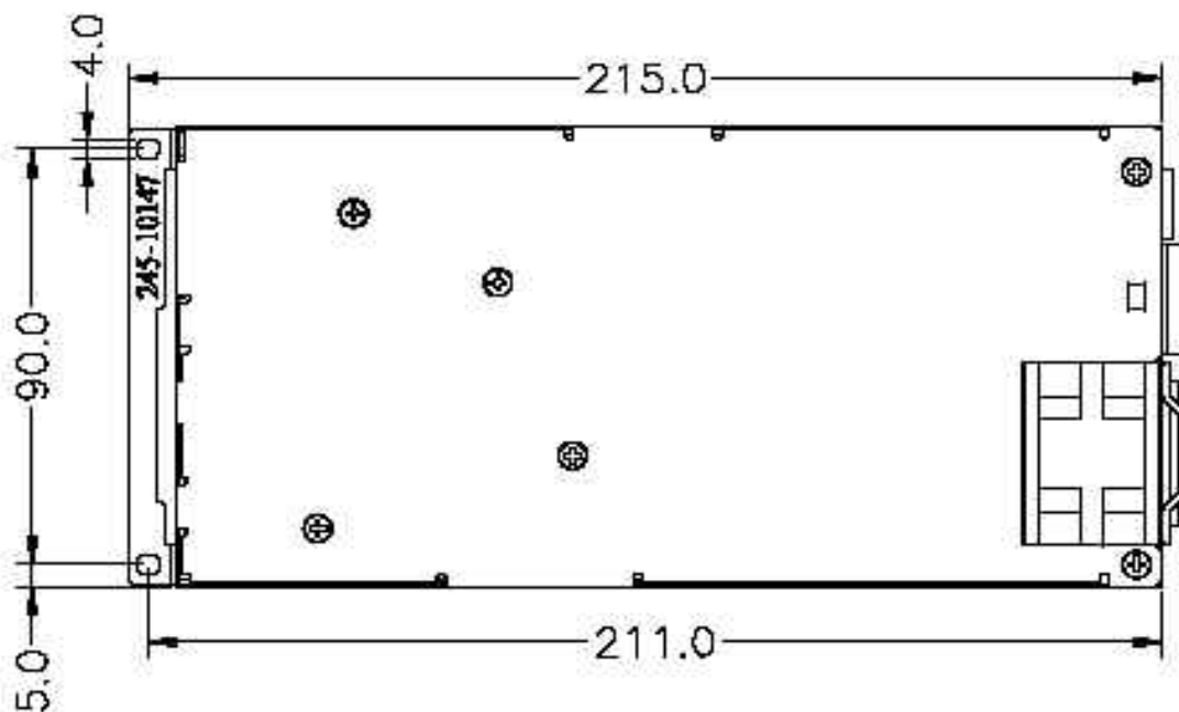
Power Supply Top View
