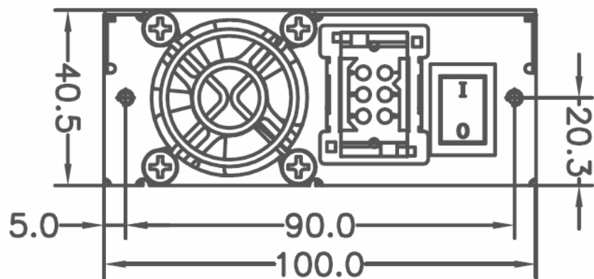
Power Supply Side View
