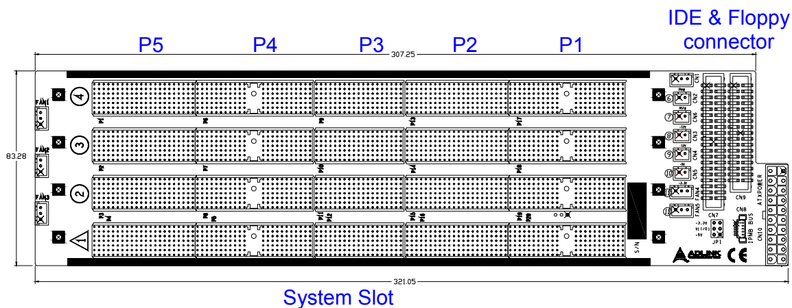
cBP-6404R/N110 Front View
