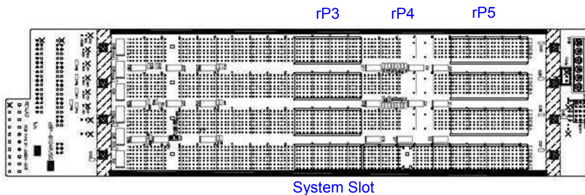
System Slot cBP-6104R Rear View
