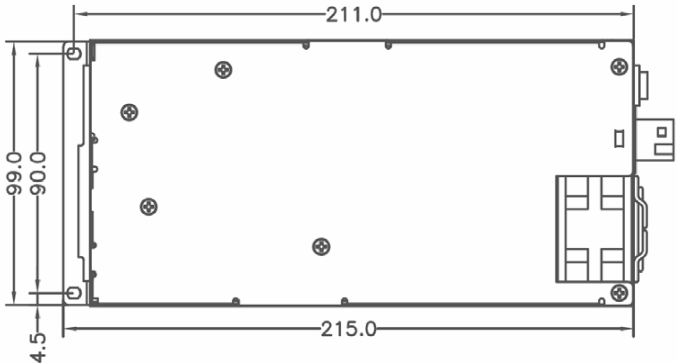
Power Supply Top View
