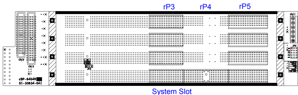
cBP-6404R Rear View
