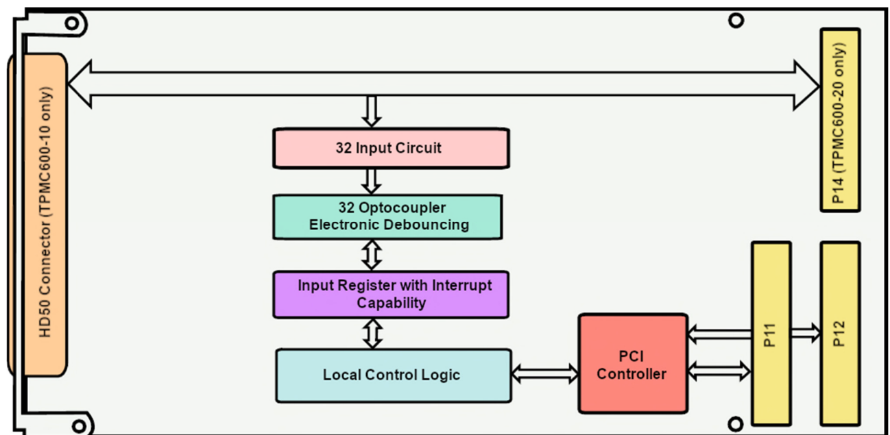
Figure 1-1 : Block Diagram
