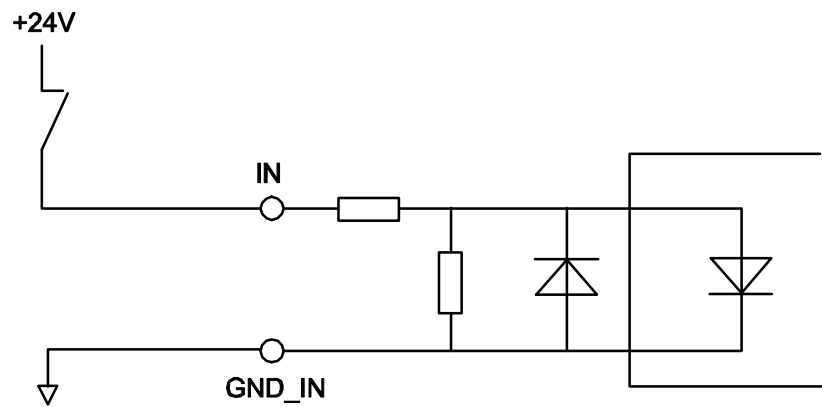
Figure 8-1 : Input Wiring
