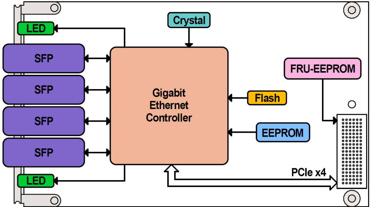
Figure 1-1 : Block Diagram
