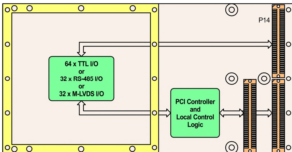
Figure 1-1 : Block Diagram
