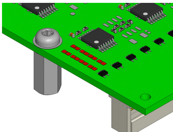
Figure 6-5 : Optional GND connection solder bridges on PCB bottom side (pads marked in red)
