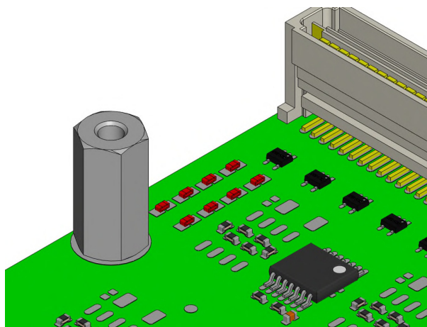
Figure 6-4 : Default 0Ω bridges on PCB top side (marked in red)
