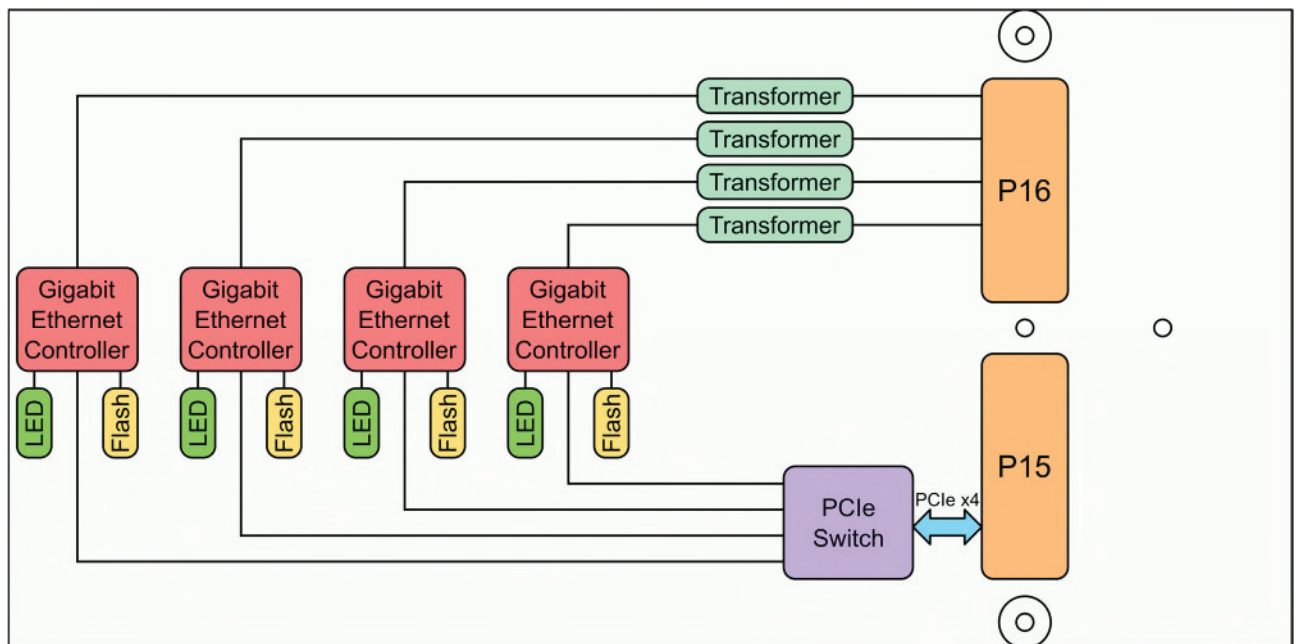
Figure 1-1 : Block Diagram
